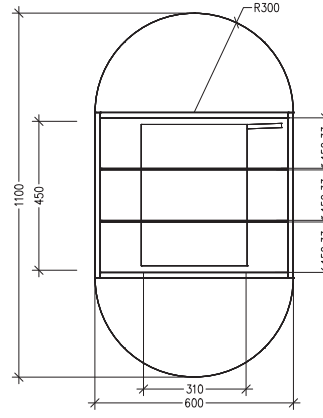
FRONT VIEW with demister
