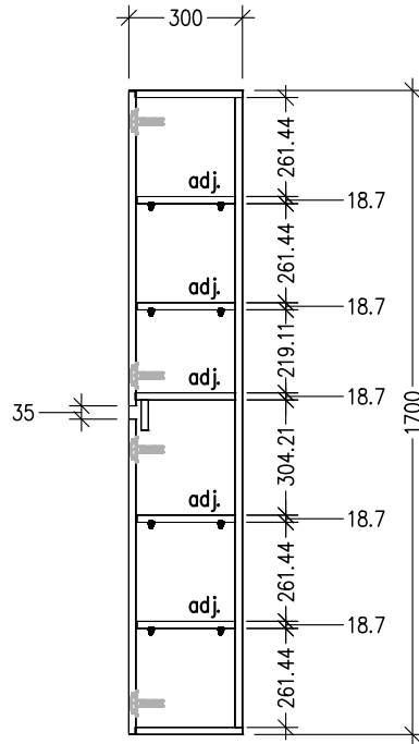
SIDE VIEW
