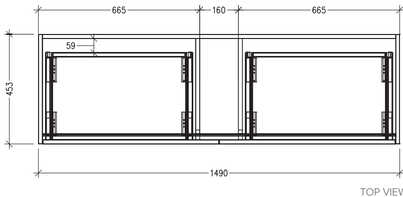
TOP VIEW
