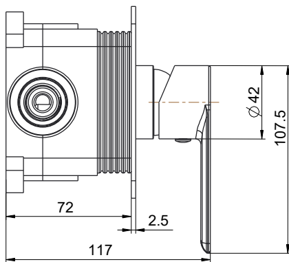
SHOWER/BATH MIXER WITH FACEPLATE & HANDLE SIDE VIEW
