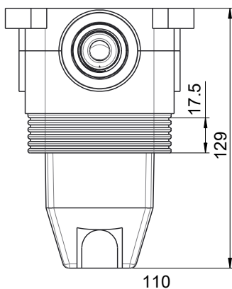
SHOWER/BATH MIXER LEAK CONTROL BOX SIDE VIEW
