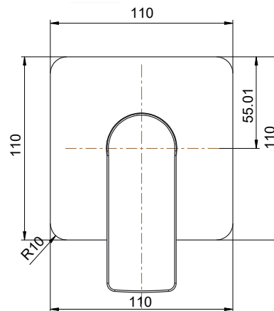
SHOWER/BATH MIXER WITH FACEPLATE & HANDLE FRONT VIEW
