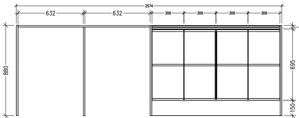
FRONT VIEW
