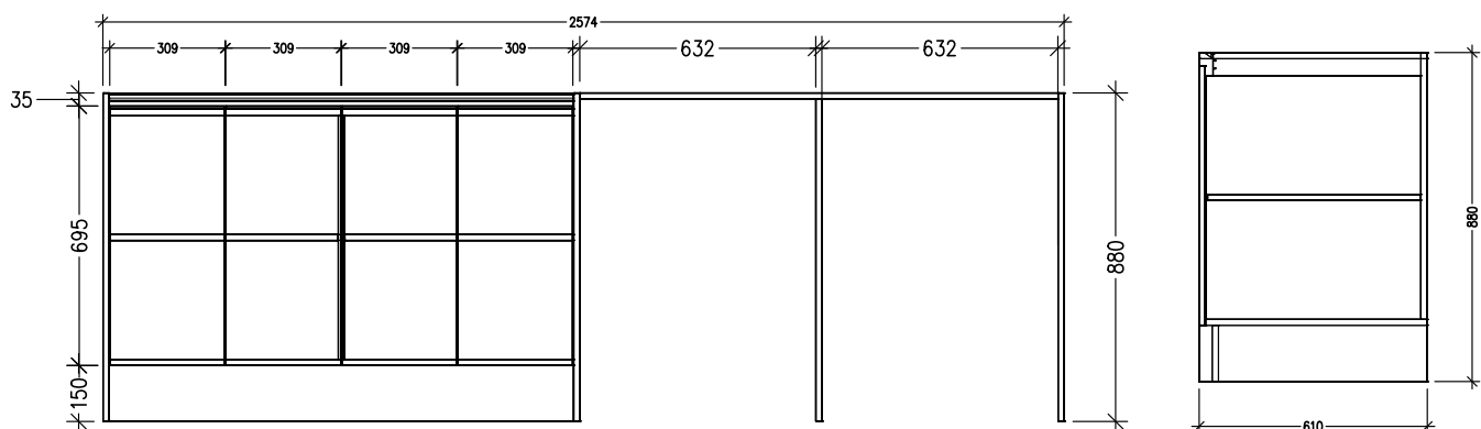
FRONT VIEW
