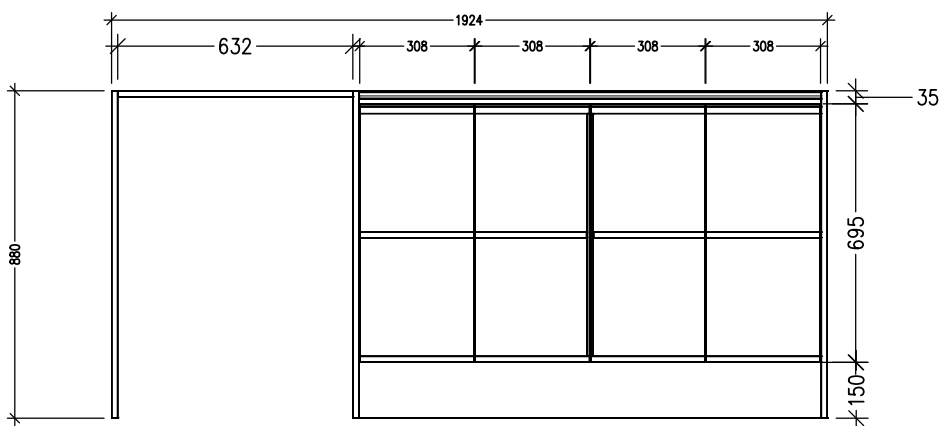
FRONT VIEW
