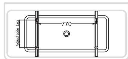
BOTTOM VIEW
