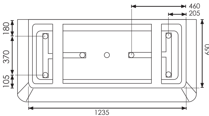
BOTTOM VIEW
