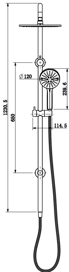
FRONT VIEW
