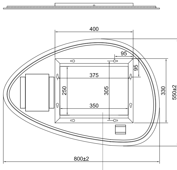
Demister Size
