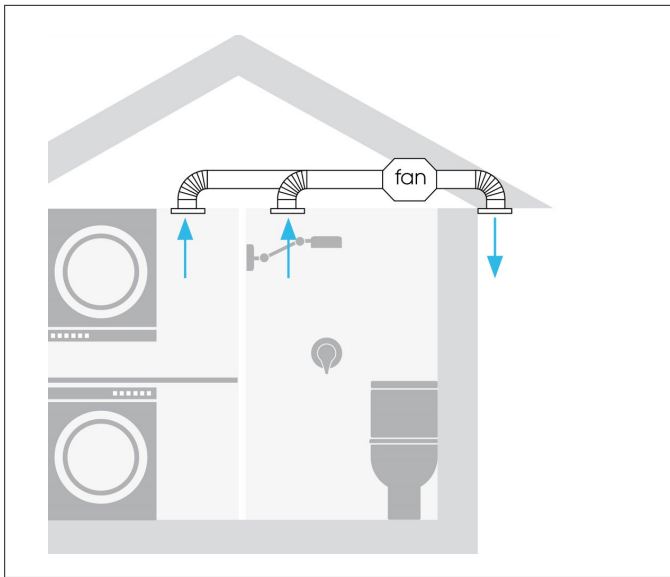
Image 1. Intake grilles not included and shown for schematic purposes. High Flow Kit allows choice of intake grilles (sold separately)
