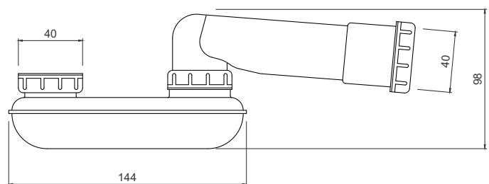
Evoke Low Profile Bath Trap [2204]
